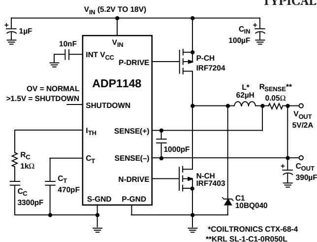
Figure 1. High Efficiency Step-Down Converter
