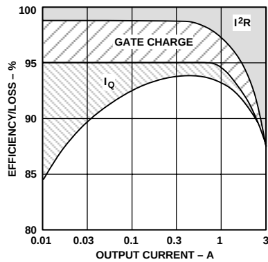
Figure 6. Typical Efficiency Losses
