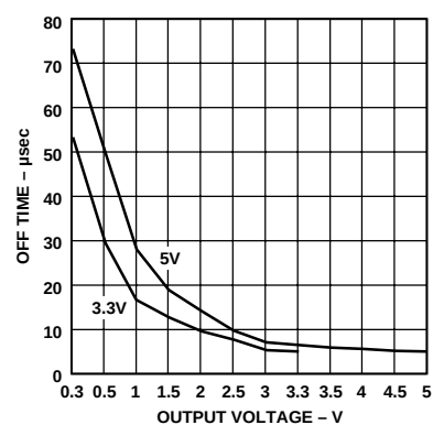
Figure 14. Off Time vs. V OUT
