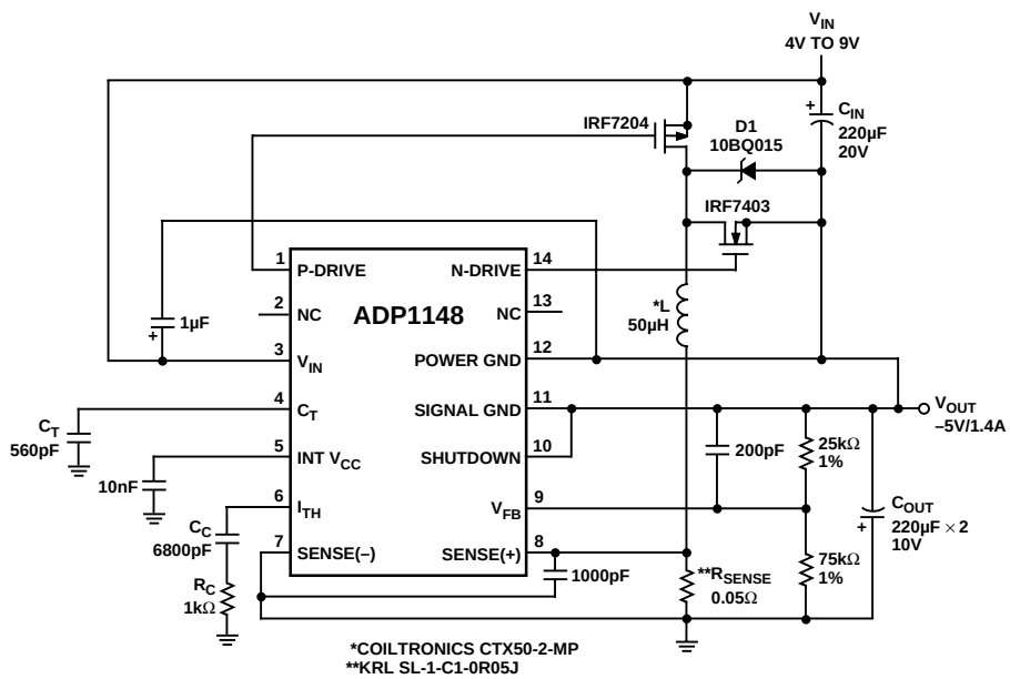
Figure 20. 4 V to 9 V Input Voltage to -5\text{ V}/1.4\text{ A} Regulator
