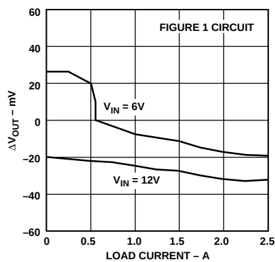
Figure 9. Load Regulation
