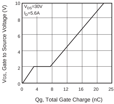
Figure 13. Gate Charge
