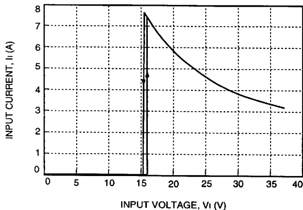
Figure 3. Typical JC100H Input Characteristics at Room Temperature, I_o = 4.2 A
