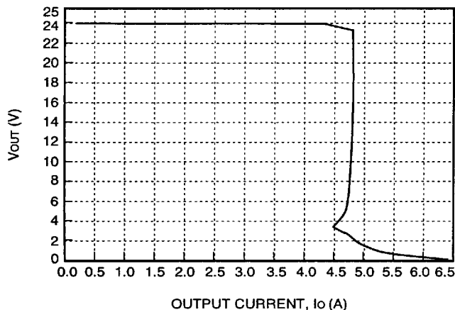
Figure 6. Typical JC100H Output Characteristics at Room Temperature, V_{IN} = 28 V
