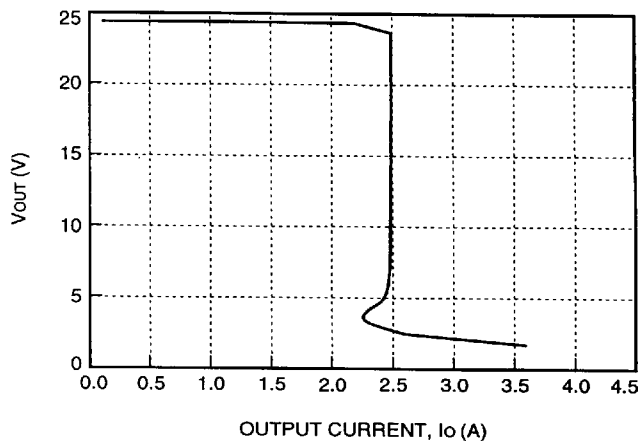
Figure 4. Typical JC050H Output Characteristics at Room Temperature, V_{IN} = 28 V
