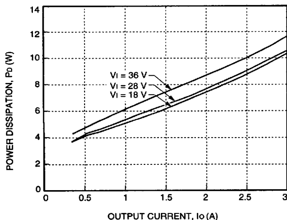
Figure 23. JC075H Power Dissipation vs. Output Current
