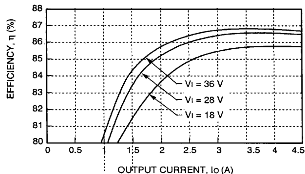
Figure 9. Typical JC100H Converter Efficiency vs. Output Current at Room Temperature
