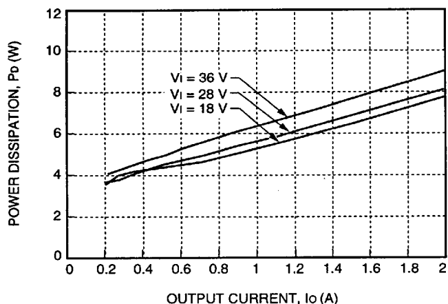
Figure 22. JC050H Power Dissipation vs. Output Current
