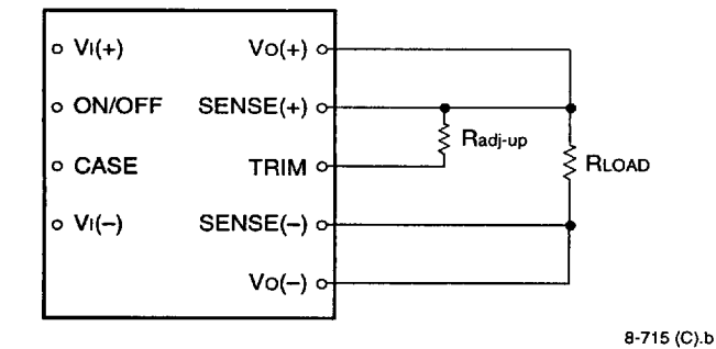
Figure 18. Circuit Configuration to Increase Output Voltage
