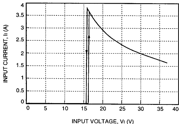
Figure 1. Typical JC050H Input Characteristics at Room Temperature, I_o = 2.1 A
