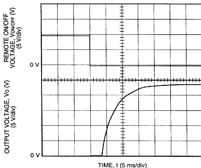
Figure 10. Typical Start-Up from Remote On/Off JCxxxH1; I_o = Full Load
