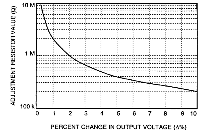
Figure 19. Resistor Selection for Increased Output Voltage 8-1294 (C)
