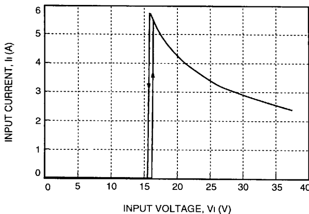
Figure 2. Typical JC075H Input Characteristics at Room Temperature, I_o = 3.1 A
