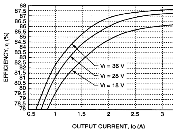
Figure 8. Typical JC075H Converter Efficiency vs. Output Current at Room Temperature
