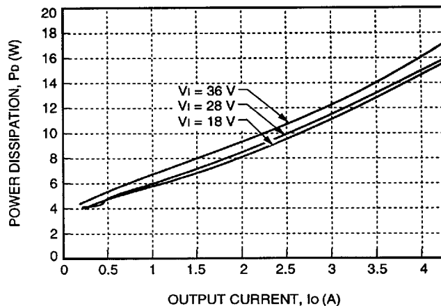
Figure 24. JC100H Power Dissipation vs. Output Current
