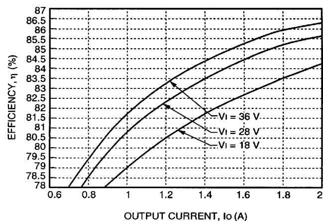
Figure 7. Typical JC050H Converter Efficiency vs. Output Current at Room Temperature
