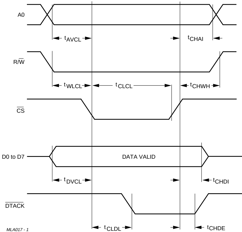
Fig.17 Bus timing (68000 mode); write cycle.
