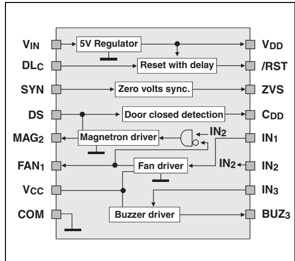
Figure 3: Block diagram
