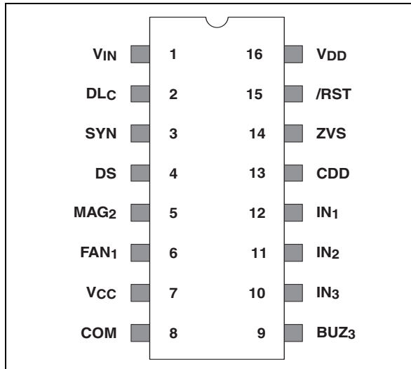
Figure 2: Pin-out connections
