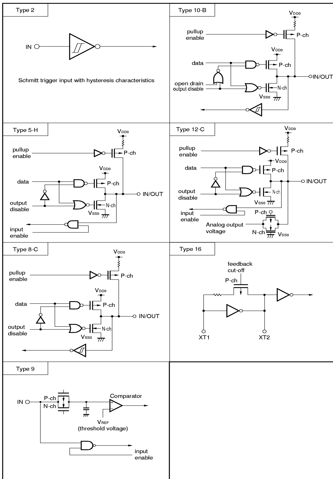
Figure 4-1. Types of Pin I/O Circuits
