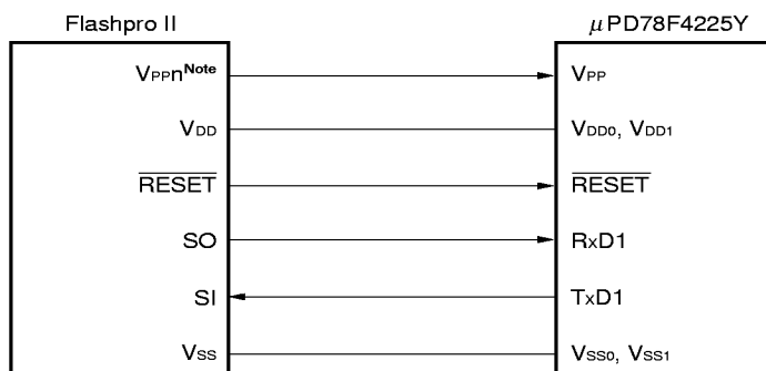
Figure 6-4. Connection of Flashpro II in UART Mode (When Using UART1)
