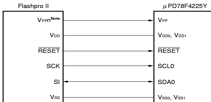
Figure 6-3. Connection of Flashpro II in I 2 C Bus Mode
