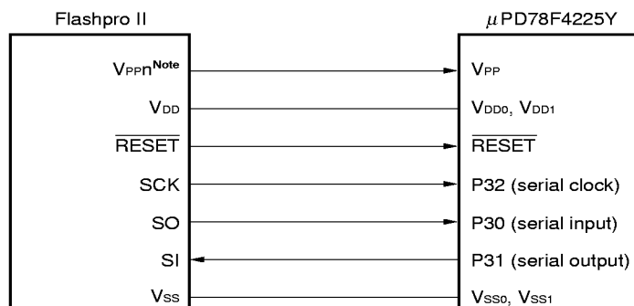
Figure 6-5. Connection of Flashpro II in Pseudo-3-Wire Serial I/O Mode
