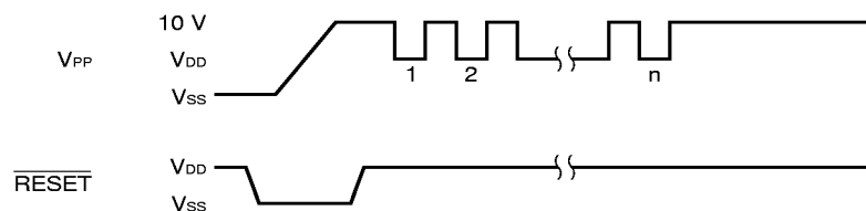
Figure 6-1. Communication Mode Selecting Format
