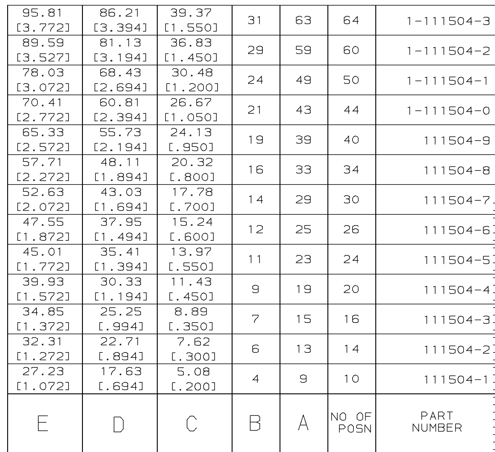
TERMINATED ASSEMBLY (ASSEMBLED BY CUSTOMER)
