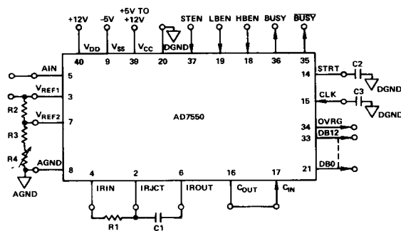
Figure 3. Operation Diagram
