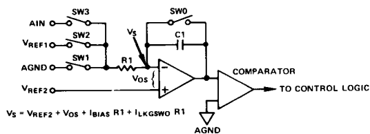
Figure 1. Quad Slope Integrator Circuit
