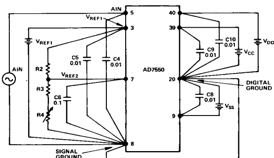
Figure 7. Ground System
