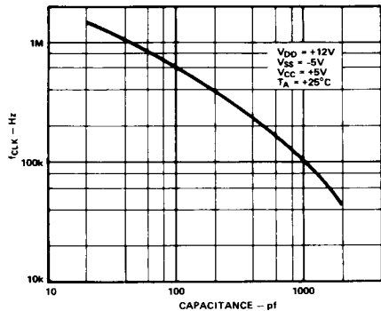
Figure 4. f_{CLK} vs. C_3
