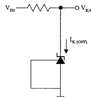
Figure 1c. Test Circuit 3
