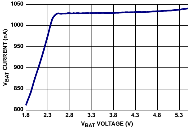
FIGURE 2. I_{BAT} vs V_{BAT} ( V_{DD}=0V )
