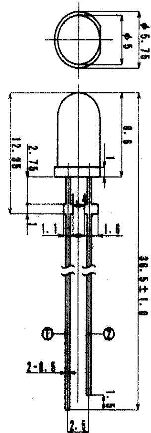
① Anode ② Cathode
