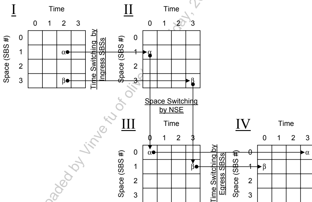
Figure 29 Time:Space:Time Switching in one NSE-8G and four Single-Ported SBSs
