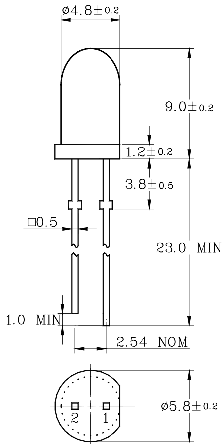
STOPPER TYPE
