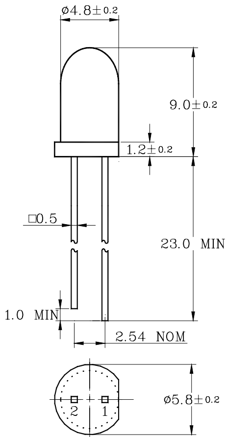
STRAIGHT TYPE
