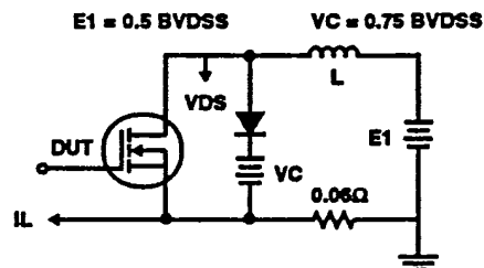
FIGURE 2. CLAMPED INDUCTIVE SWITCHING
