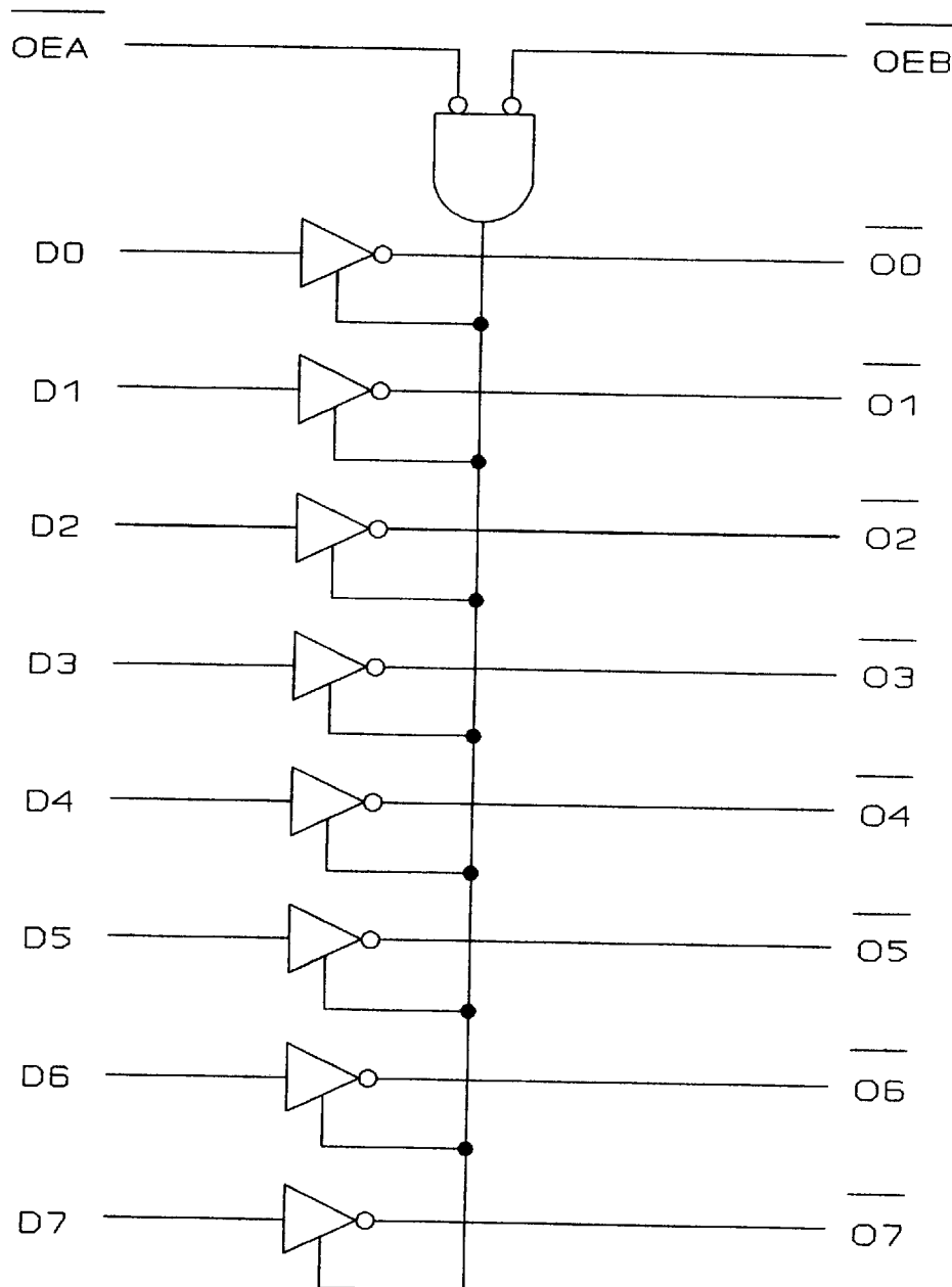
FIGURE 3. Logic diagram.
