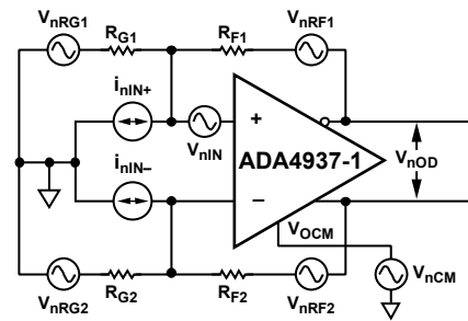
Figure 47. ADA4937-1 Noise Model
