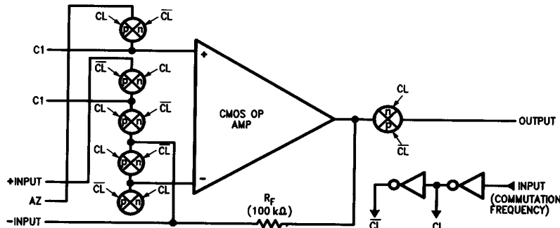
Figure 6: Schematic of Analog Switches Connecting Each Internal OP AMP to the External Inputs and Output
