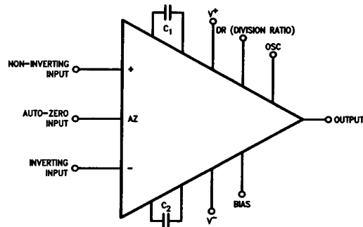
Figure 3: Symbol
