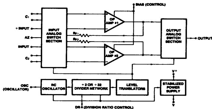
Figure 2: Functional Diagram
