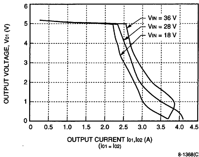
Figure 2. LC016AJ Typical Output Characteristics, T_A = 25^\circ\text{C}
