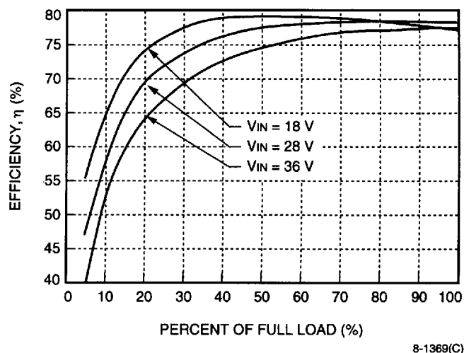
Figure 3. LC016AJ Typical Converter Efficiency vs. Output Current, T_A = 25^\circ\text{C}
