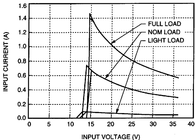
Figure 1. LC016AJ Typical Input Characteristics, T_A = 25^\circ\text{C}
