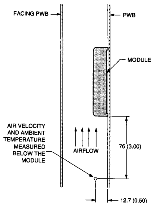
Figure 14. Experimental Test Setup
