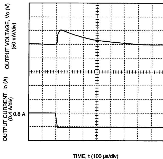
Figure 4. LC016AJ Typical Output Voltage for a Step Load Change from 50% to 25%
