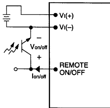
Figure 10. Remote On/Off Implementation
