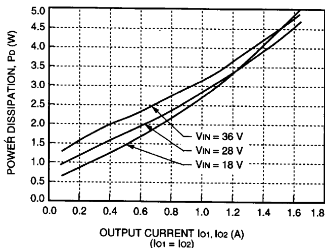
Figure 13. LC016AJ Power Dissipation vs. Output Current, T_A = 25^\circ\text{C}
