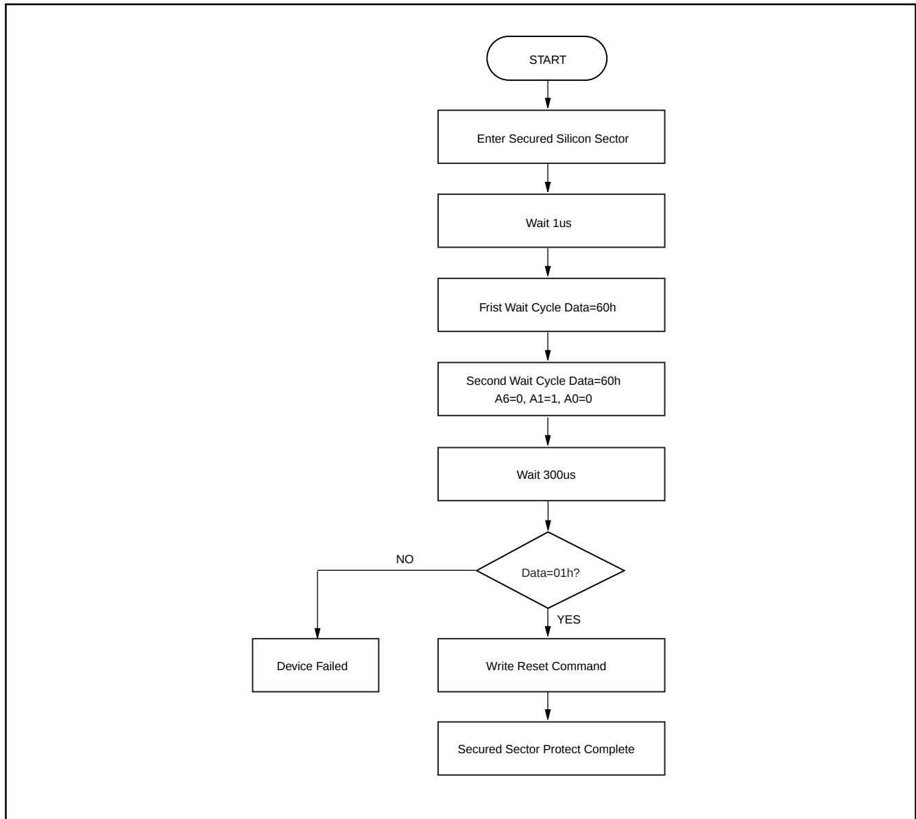
Fig 10. SECURED SILICON SECTOR PROTECTED ALOGORITHMS FLOWCHART
