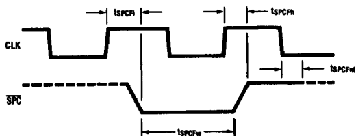
FIGURE 4-9. SPC Pulse from FPU
