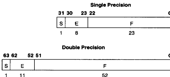
FIGURE 1-1. Floating-Point Operand Formats
