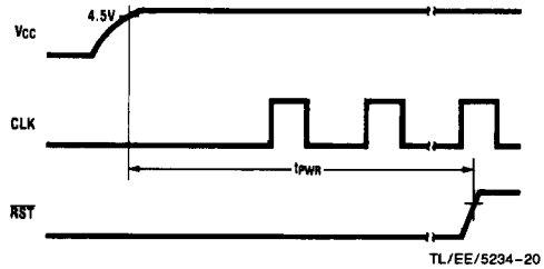
FIGURE 4-5. Power-On Reset
