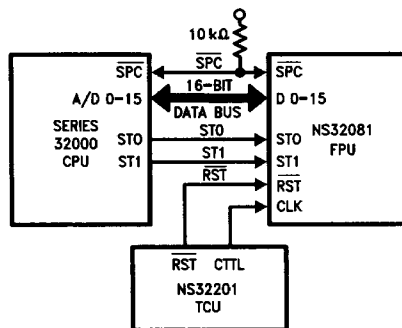
FIGURE 3-4. System Connection Diagram
