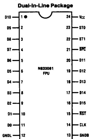
Top View FIGURE 4-1. Connection Diagram
