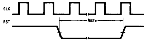
FIGURE 4-6. Non-Power-On Reset
