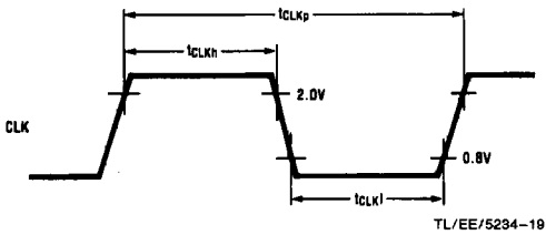
FIGURE 4-4. Clock Timing
