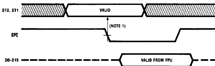
FIGURE 3-5. Slave Processor Read Cycle
