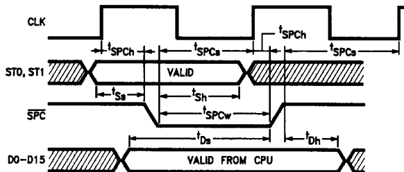
FIGURE 4-8. Write Cycle to FPU
