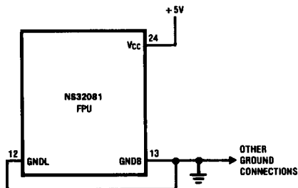
FIGURE 3-1. Recommended Supply Connections
