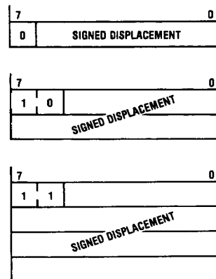
FIGURE 2-5. Displacement Encodings
