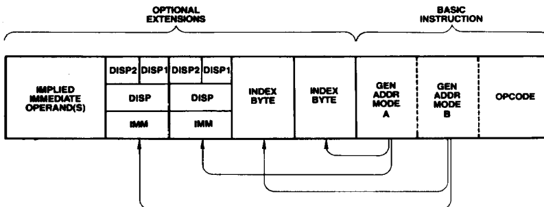
FIGURE 2-3. General Instruction Format
