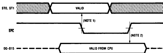
FIGURE 3-6. Slave Processor Write Cycle
