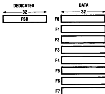
FIGURE 2-1. Register Set
