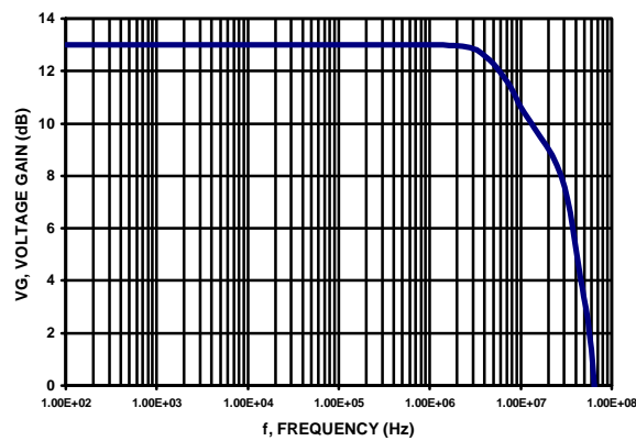
Figure 5 . Frequency Response
