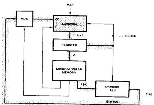
Figure 4. Address-Based Architecture
