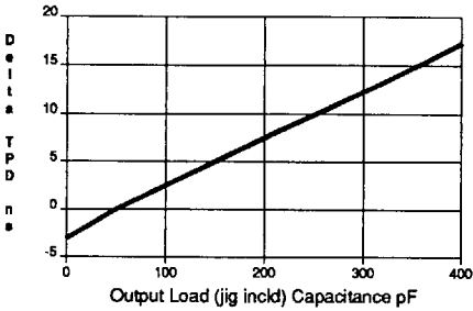
DELTA TPD vs. OUTPUT LOADING
