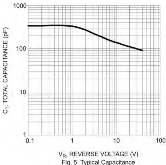
Fig. 5 Typical Capacitance
