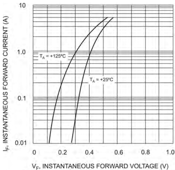
Fig. 3 Typ. Forward Characteristics - B350B thru B360B
