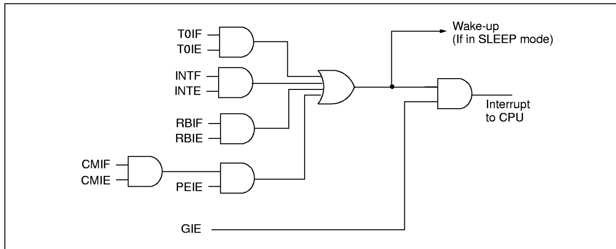
FIGURE 9-16: INTERRUPT LOGIC
