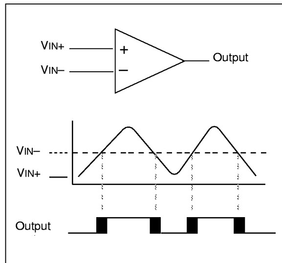
FIGURE 7-2: SINGLE COMPARATOR
