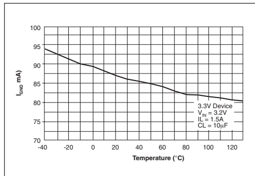
Figure 13. Ground Current vs Temperature in Dropout at I_{LOAD} = 1.5A
