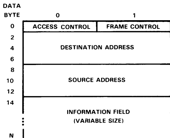
FIGURE 5. TRANSMIT DATA FORMAT
