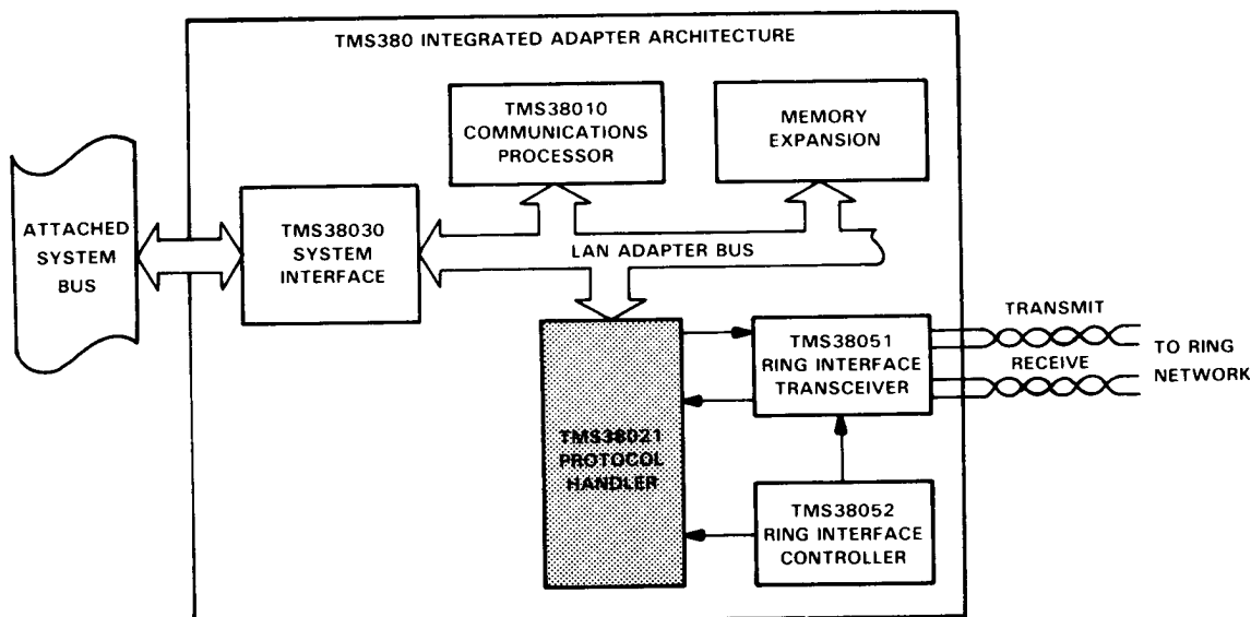
token ring LAN application diagram
