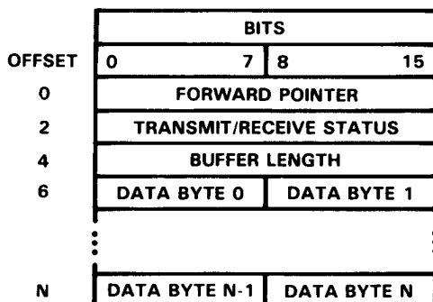
FIGURE 4. BUFFER ORGANIZATION
