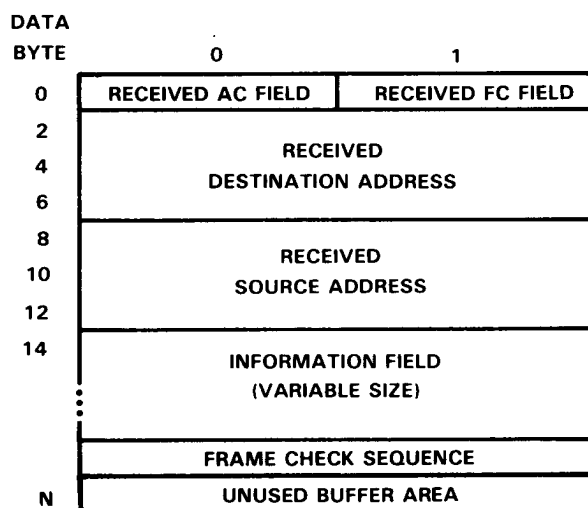
FIGURE 6. RECEIVE DATA FORMAT
