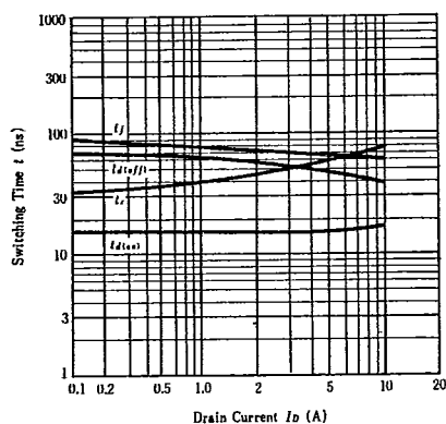
SWITCHING CHARACTERISTICS
