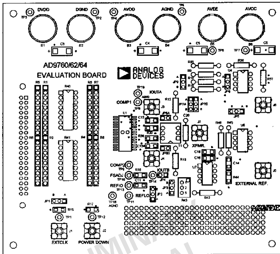
Figure 40. Silkscreen Layer—Top
