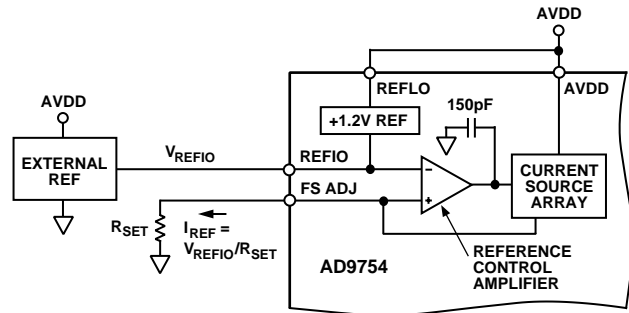
Figure 23. External Reference Configuration
