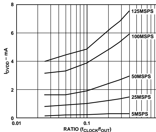
Figure 30. I_{DVDD} vs. Ratio @ DVDD = 3 V
