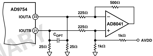
Figure 33. Single-Supply DC Differential Coupled Circuit
