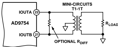
Figure 31. Differential Output Using a Transformer
