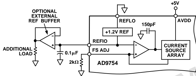
Figure 22. Internal Reference Configuration
