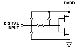
Figure 27. Equivalent Digital Input
