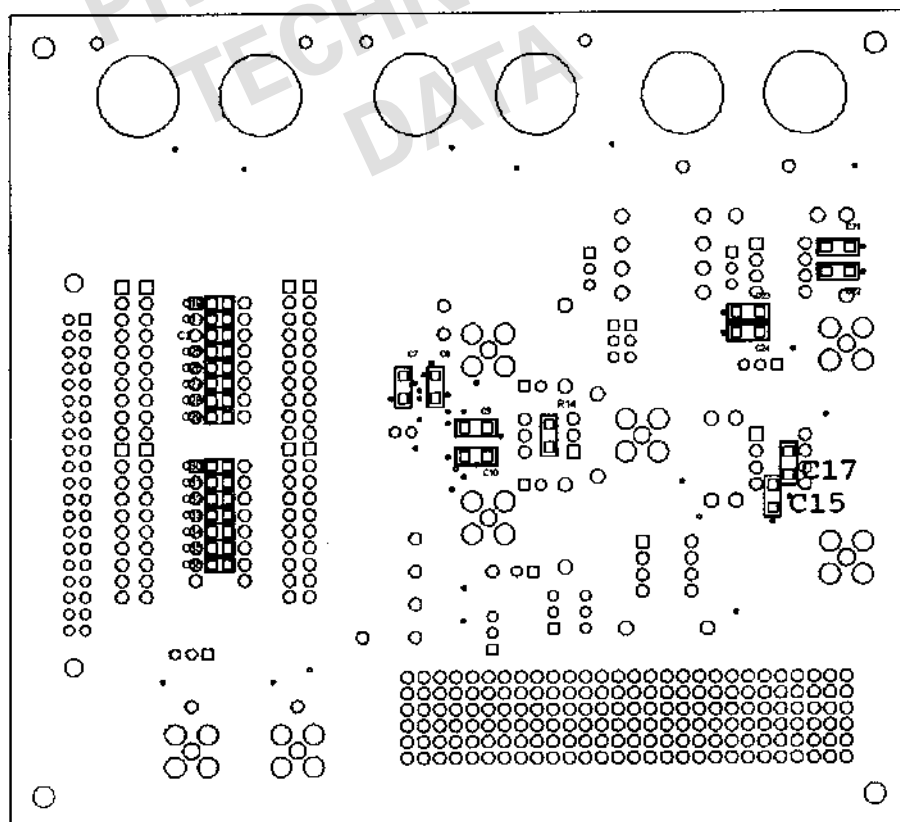
Figure 45. Silkscreen Layer—Bottom
