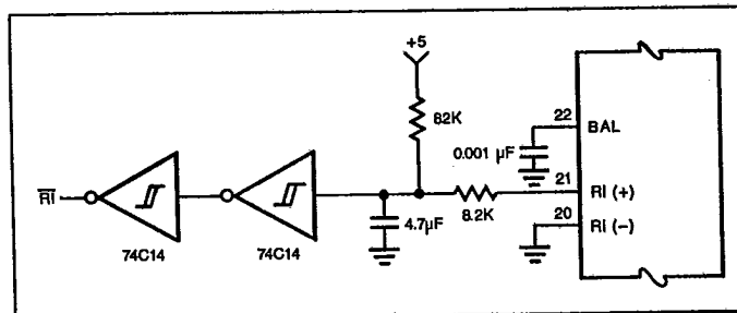
Figure 3a. Ring Envelope Detect
