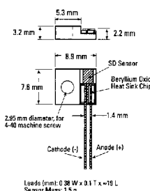
Leads (mm): 0.38 W x 0.17 x ~10 L Sensor Mass: 1.5 g
