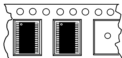
Feed Direction Typical SSOP, TSSOP Package Orientation
