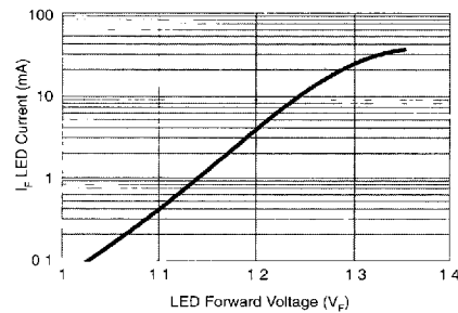
2) LED Forward Current ( I_F ) vs. Forward Voltage ( V_F )
