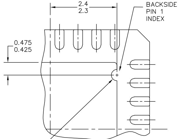
DETAIL M BACKSIDE PIN 1 INDEX OPTION
