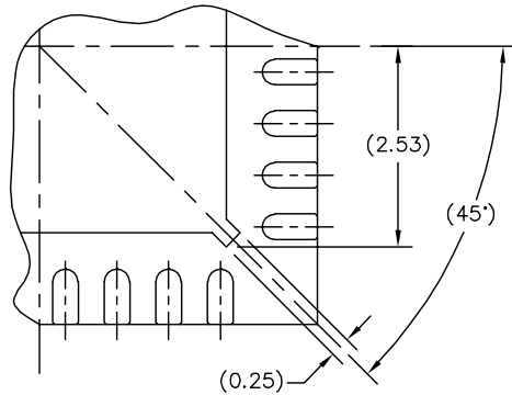
DETAIL N PREFERRED CORNER CONFIGURATION
