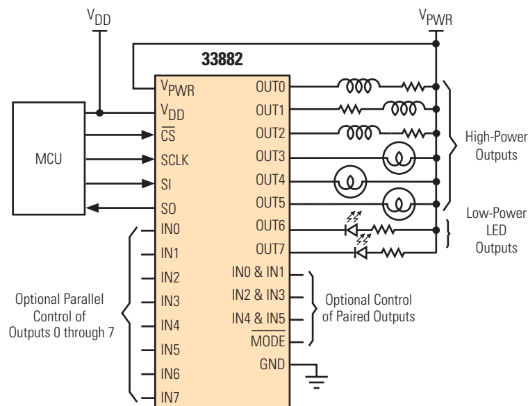
Figure 1. 33882 Simplified Application Diagram
