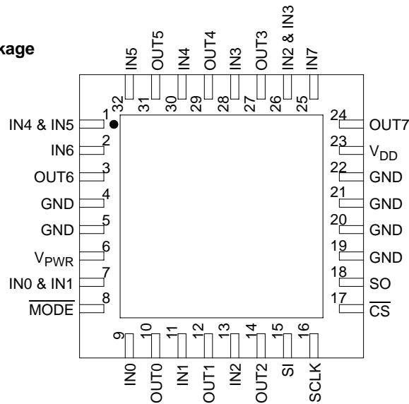
Figure 4. QFN Pin Connections
