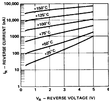
Figure 13. (5082-2835) Typical Variation of Reverse Current ( I_R ) vs. Reverse Voltage ( V_R ) at Various Temperatures.
