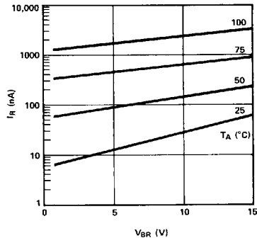
Figure 2. 5082-2300 Series Typical Reverse Current vs. Reverse Voltage at Various Temperatures.
