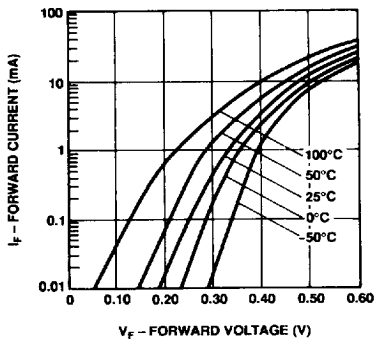
Figure 1. I-V Curve Showing Typical Temperature Variation for 5082-2300 and 5082-2900 Series Schottky Diodes.
