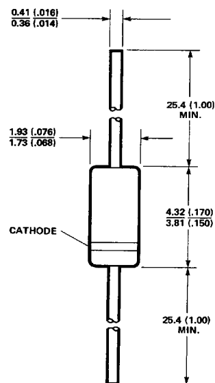
DIMENSIONS IN MILLIMETERS AND (INCHES).
