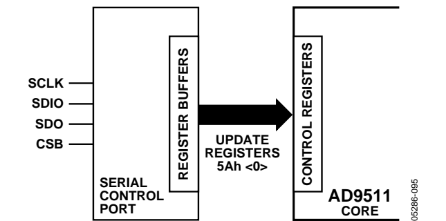
Figure 45. Relationship Between Serial Control Port Register Buffers and Control Registers of the AD9511
