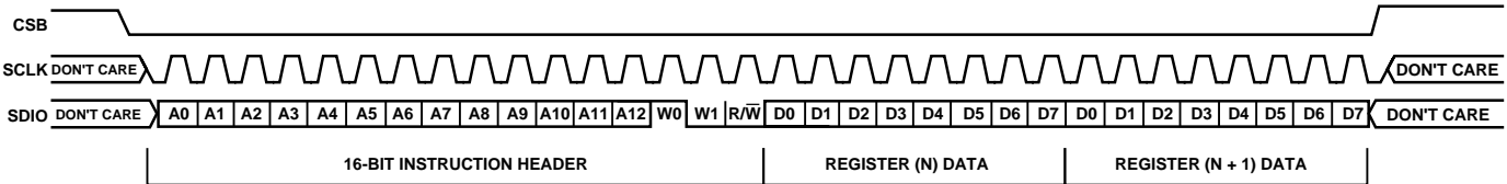
Figure 50. Serial Control Port Write—LSB First, 16-Bit Instruction, 2 Bytes of Data
