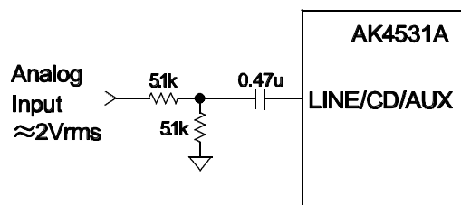
Figure 4. 2Vrms Line level Input
