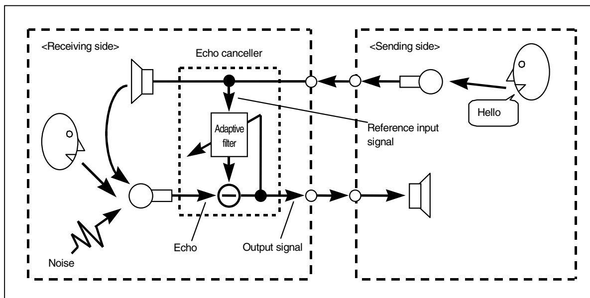
Figure 1-1. Concept of Echo Canceller
