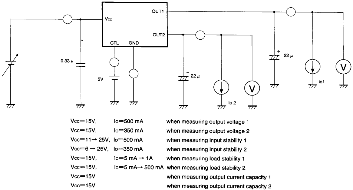
Fig.1 Circuit for measuring output voltage, line regulation, load regulation, and output current capacity
