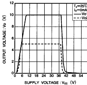
Fig.9 Output vs. supply voltage (typ.)
