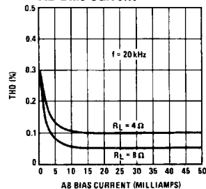
Total Harmonic Distortion vs AB Bias Current
