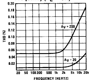
Total Harmonic Distortion vs Frequency ( R_L = 8\Omega )
