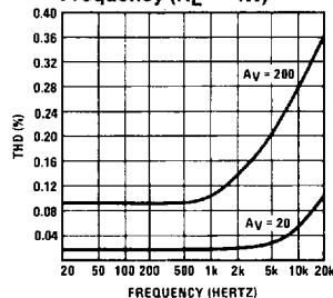
Total Harmonic Distortion vs Frequency ( R_L = 4\Omega )
