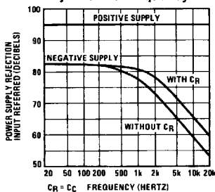
Input Referred Power Supply Rejection vs Frequency
