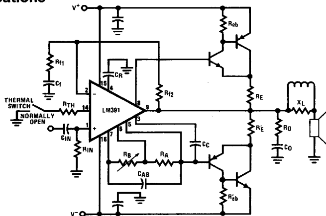
FIGURE 1. LM391 with External Components—Protection Circuitry Not Shown
