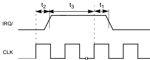
Figure 6.10 Interrupt Output
