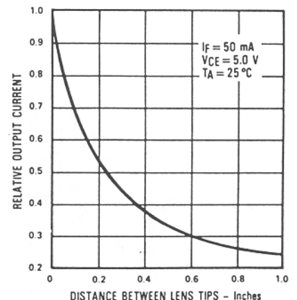
Coupling Characteristics OP165 and OP505
