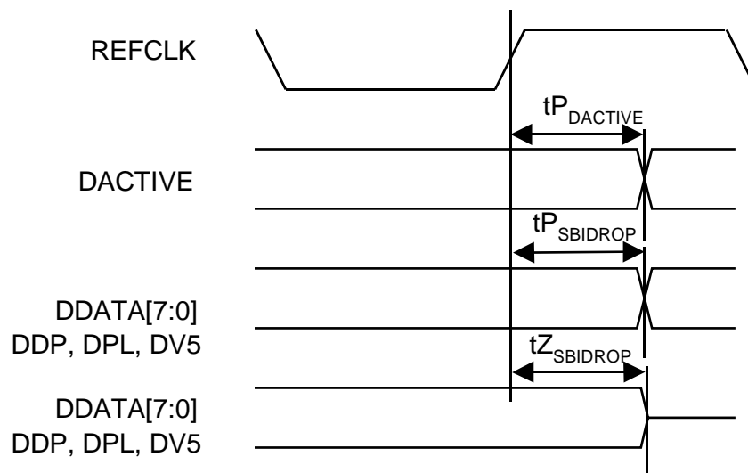
Figure 32 SBI DROP BUS Timing
