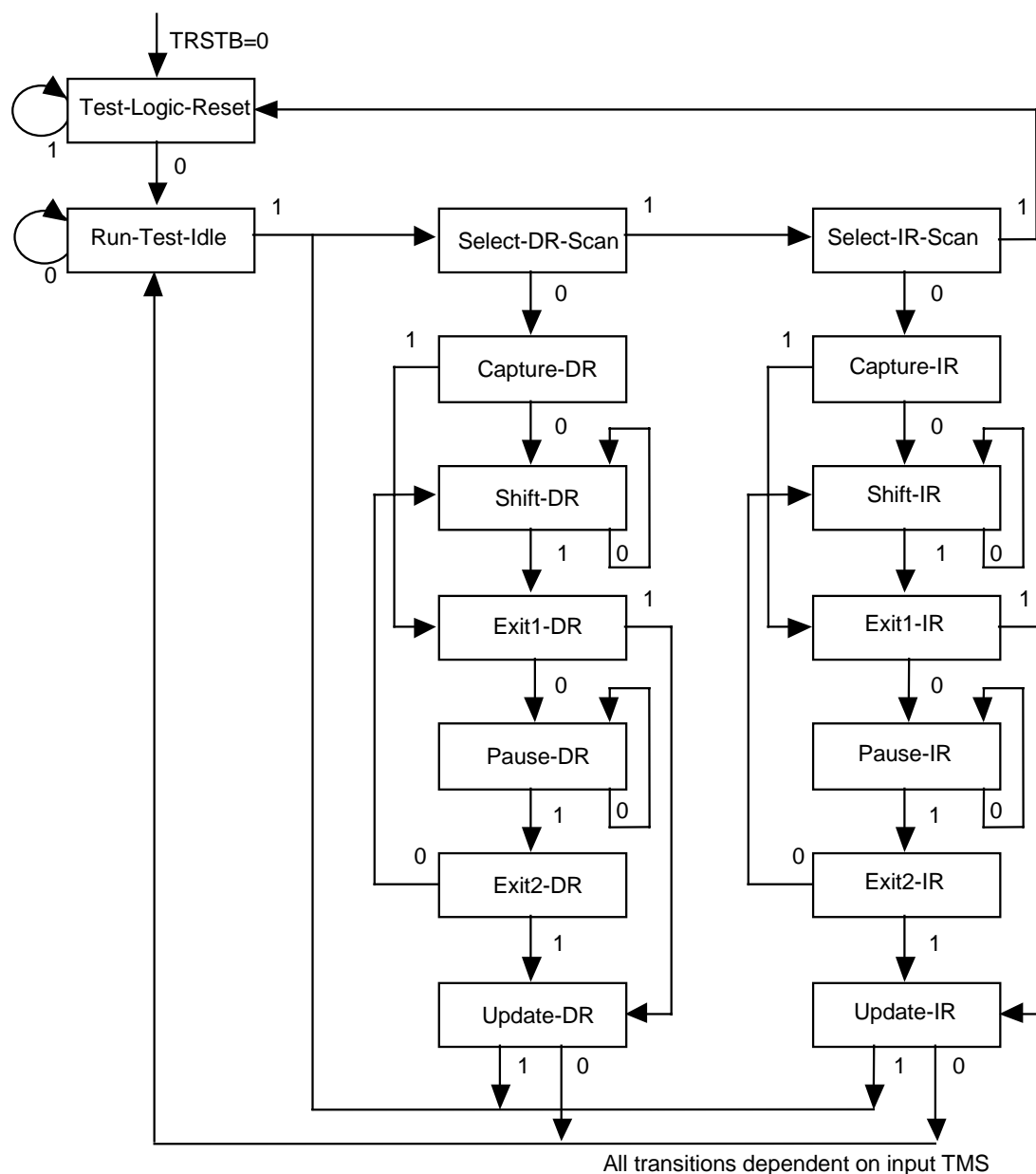
Figure 16 TAP Controller Finite State Machine
