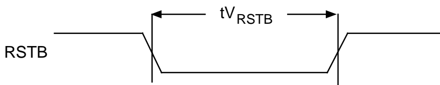
Figure 28 RSTB Timing
