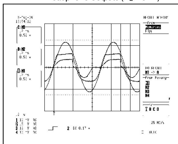
Figure 4 : Maximum Voltage Swing at Headphone Outputs ( R_L = 32\Omega )
