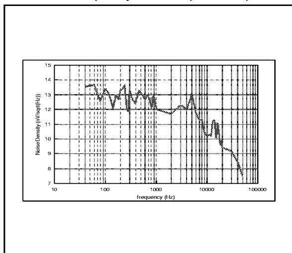
Figure 3 : Voltage Noise Density versus Frequency at Preamplifier Output
