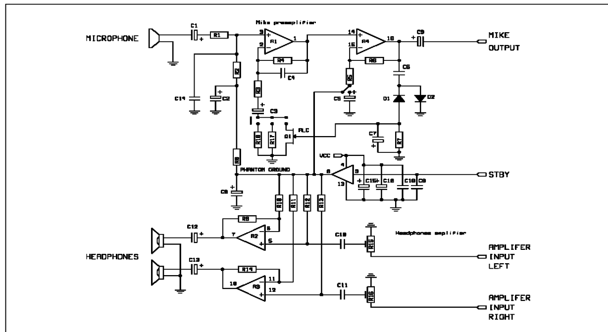
Figure 1 : Electrical Schematic
