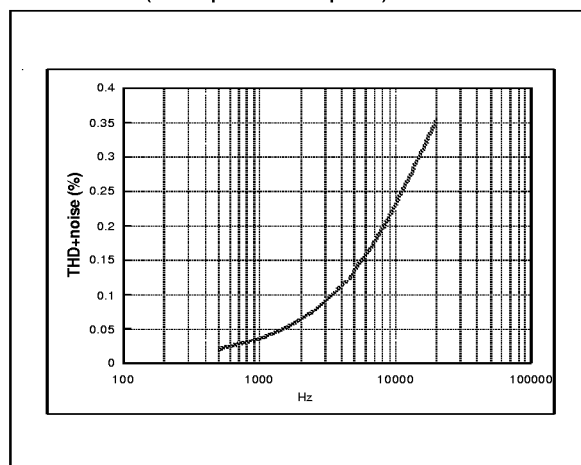
Figure 5 : THD+Noise versus Frequency (headphone outputs)
