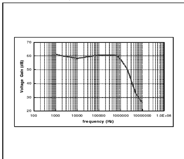
Figure 2 : Frequency Response of the Global Preamplifier Chain
