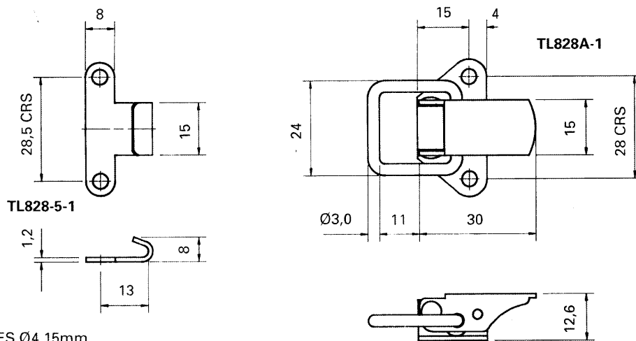
FIXING HOLES Ø4,15mm
