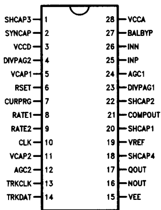
28-Pin Molded DIP
