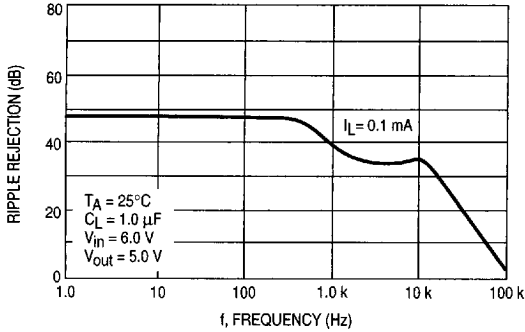
Figure 11. Ripple Rejection
