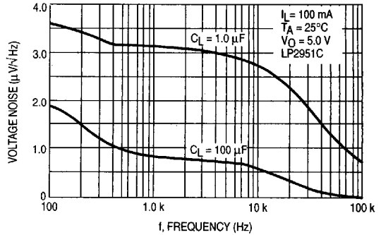
Figure 12. Output Noise
