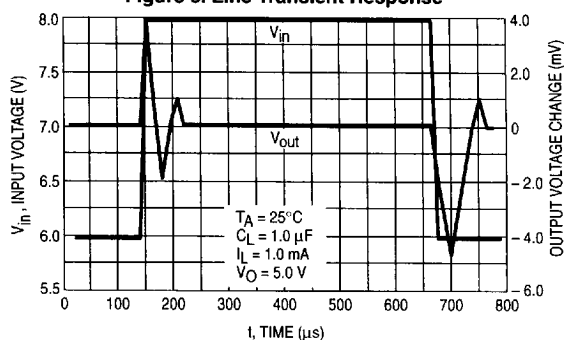
Figure 8. Line Transient Response
