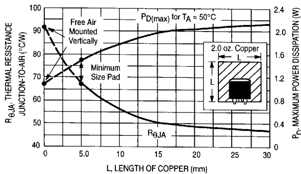
Figure 26. DPAK Thermal Resistance and Maximum Power Dissipation versus P.C.B. Copper Length
