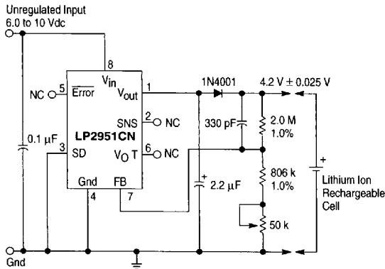
Figure 18. Lithium Ion Battery Cell Charger
