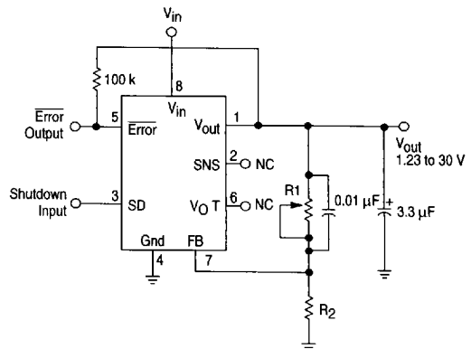
Figure 16. Adjustable Regulator
