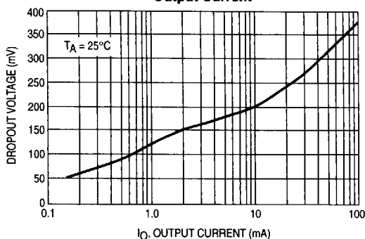
Figure 5. Dropout Voltage versus Output Current
