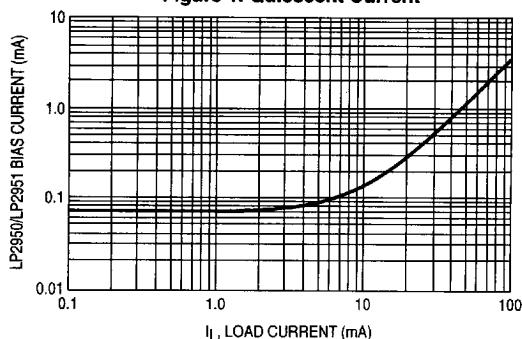
Figure 1. Quiescent Current
