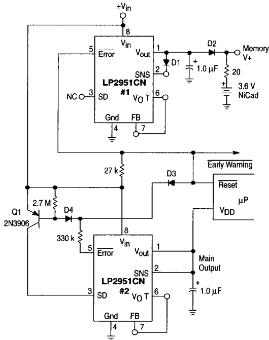
Figure 22. Regulator with Early Warning and Auxiliary Output
