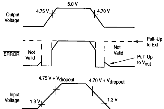
Figure 15. ERROR Output Timing
