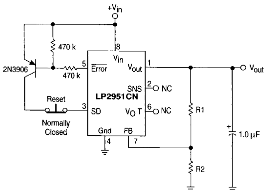
Figure 20. Latch Off When Error Flag Occurs
