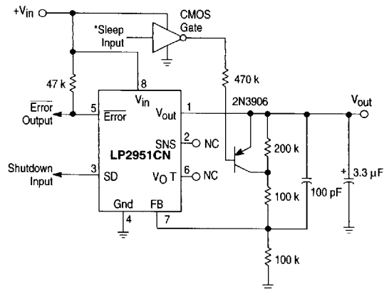
Figure 21. 5.0 V Regulator with 2.5 V Sleep Function
