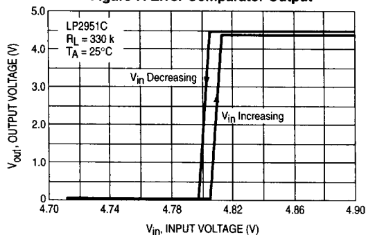
Figure 7. Error Comparator Output
