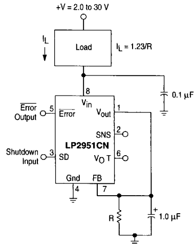
Figure 19. Low Drift Current Sink
