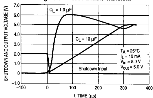
Figure 9. LP2951 Enable Transient
