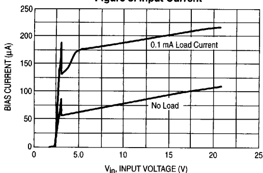
Figure 3. Input Current
