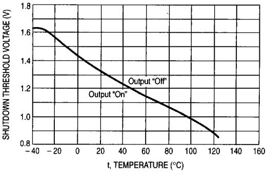
Figure 13. Shutdown Threshold Voltage versus Temperature
