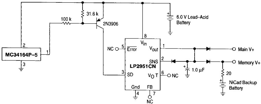
Figure 25. Low Battery Disconnect
