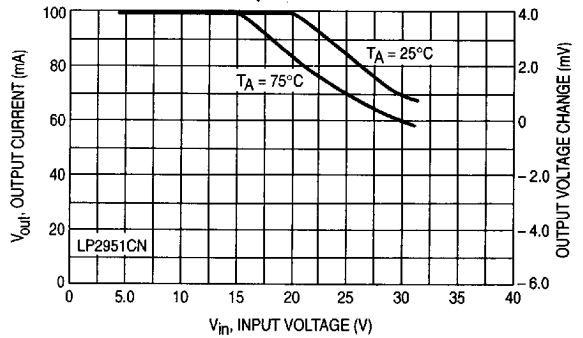
Figure 14. Maximum Rated Output Current
