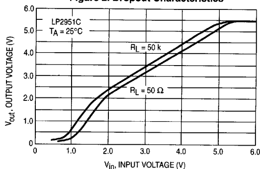
Figure 2. Dropout Characteristics
