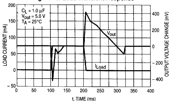
Figure 10. Load Transient Response
