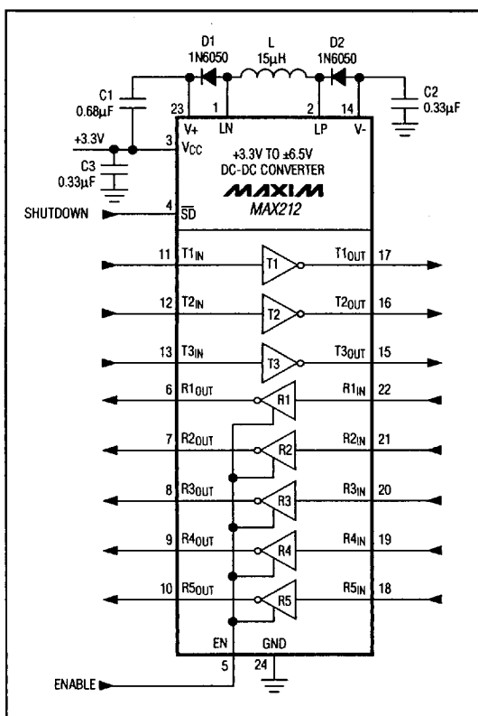
Figure 1. Typical Application Circuit
