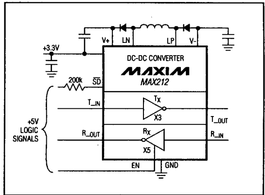
Figure 2. Connecting to +5V Logic
