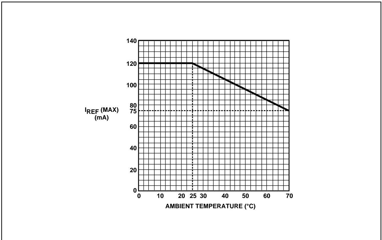
Fig.6 Derating curve
