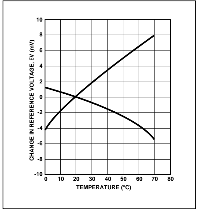
Fig.5 Temperature characteristic (typical)
