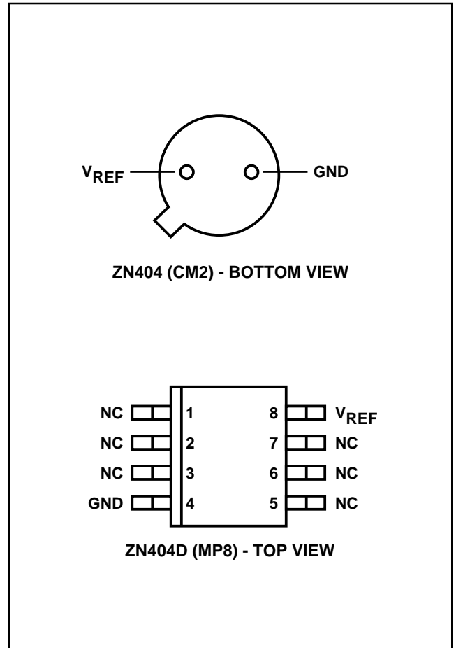
Fig.1 Pin connections
