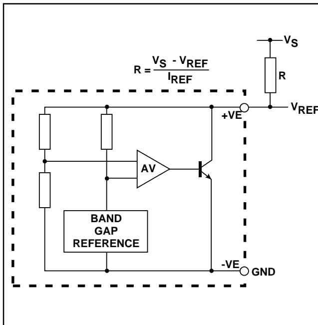
Fig.2 Circuit diagram
