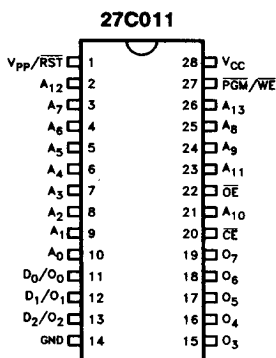
Figure 2. Pin Configuration
