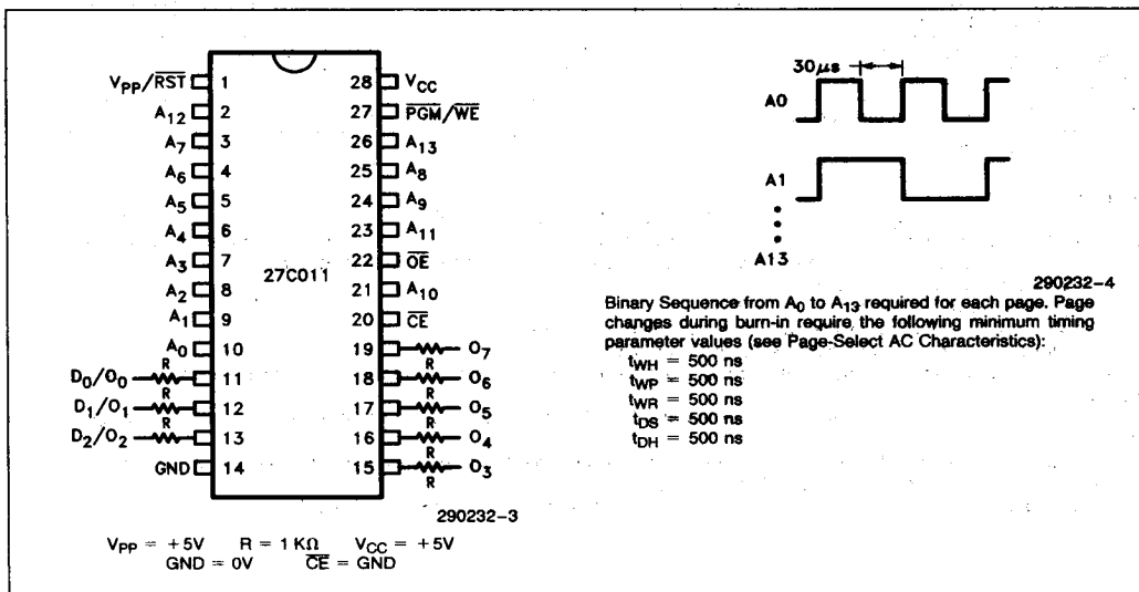
Burn-In Bias and Timing Diagrams
