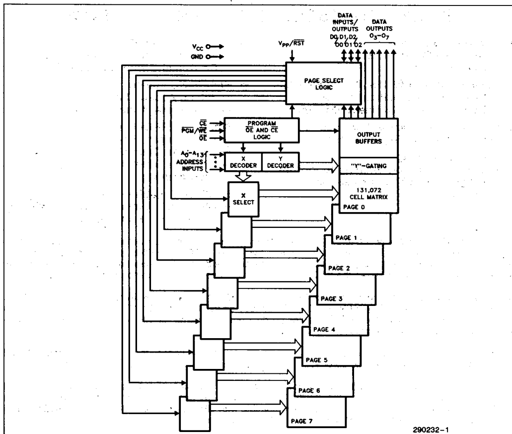
Figure 1. Block Diagram
